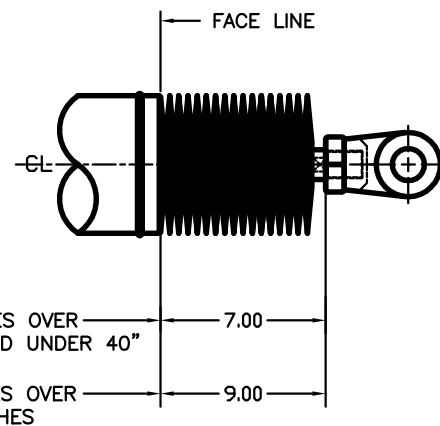
SHOWN WITH ROD/BOOT FULLY RETRACTED STROKES OVER 24 INCHES
