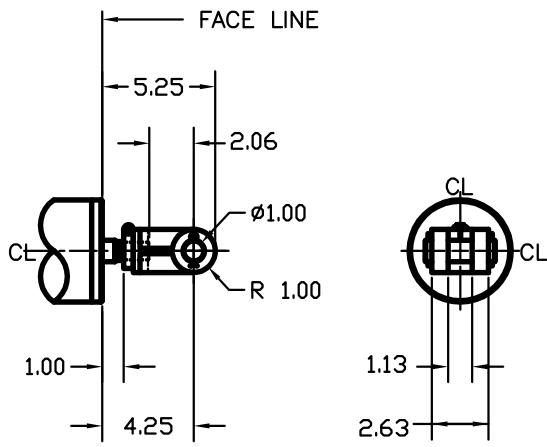
FEMALE CLEVIS WITH PIN
